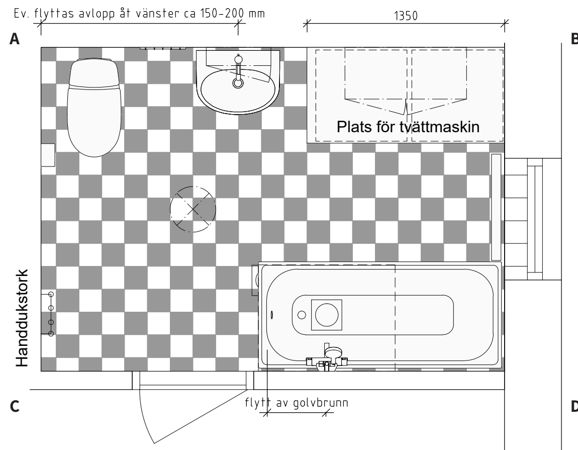
Plan
